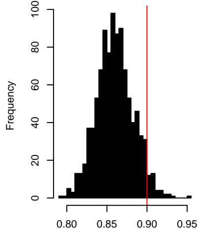
H distribution – H = 0.9
