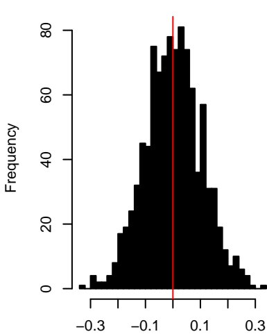
Mu distribution – H = 0.7
