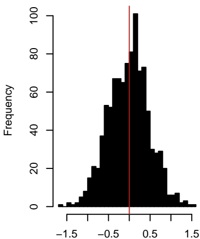
Mu distribution – H = 0.9
