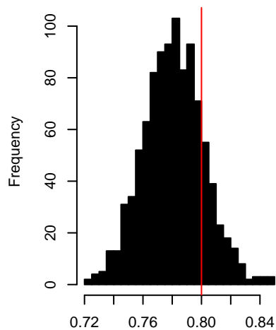
H distribution – H = 0.8
