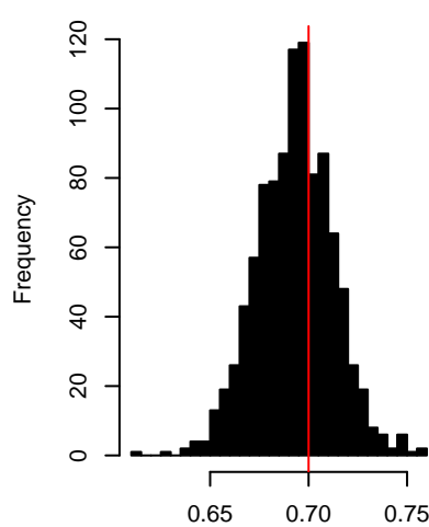
H distribution – H = 0.7
