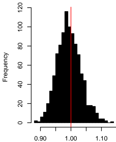
Sigma distribution – H = 0.7
