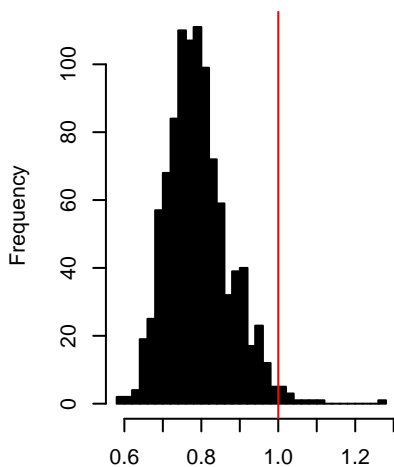
Sigma distribution – H = 0.9
