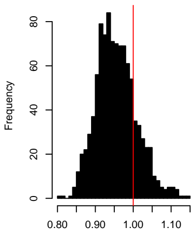
Sigma distribution – H = 0.8
