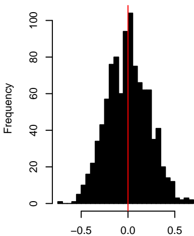
Mu distribution – H = 0.8
